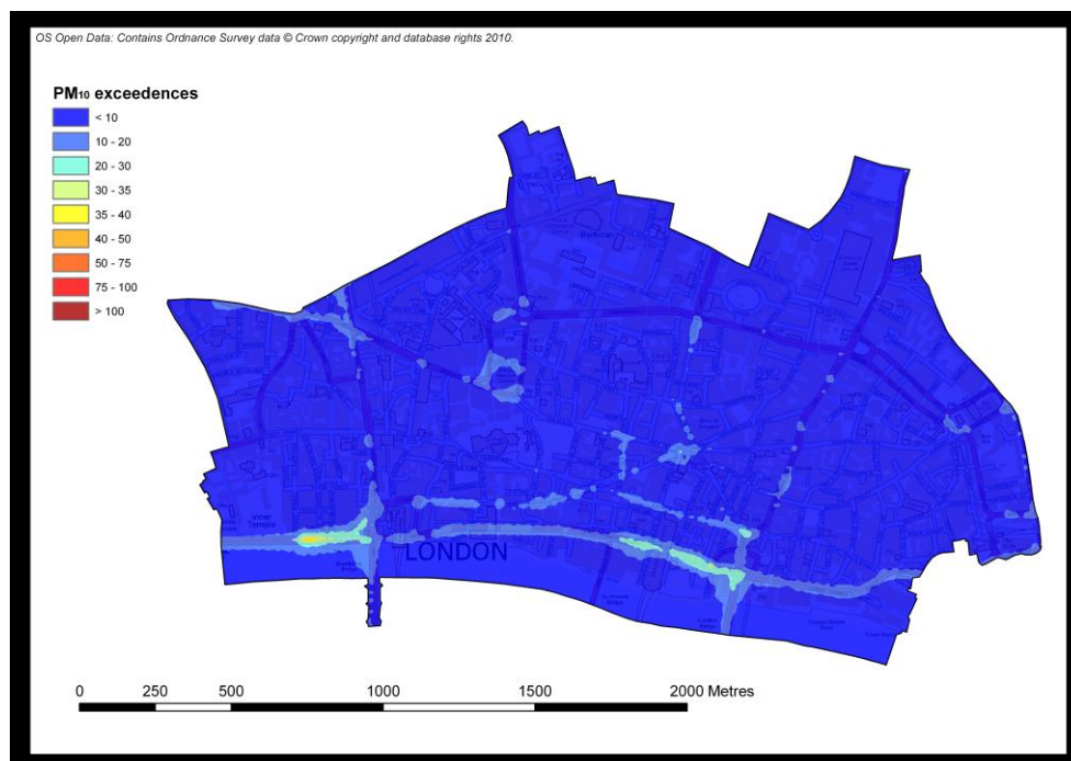
Figure 3.6: Modelled concentrations of daily average PM 10 exceedences, 2015
